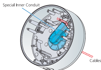
Water-resistant Design (SNC-DF80 inside)
